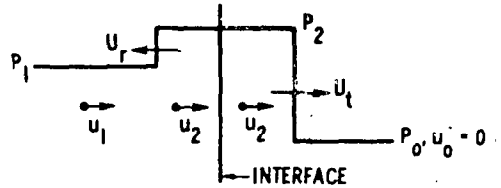
(c) PRESSURE-DISTANCE PROFILE AFTER INTERACTION
